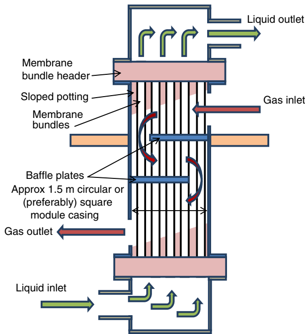
Figure 3 Detailed schematic of a possible design of a HFMM and internals.
