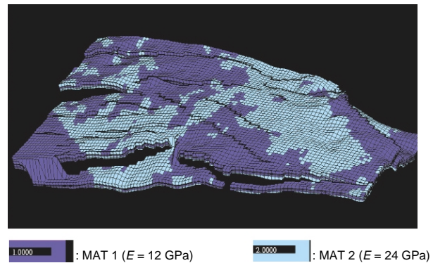
Figure 11 Material mechanical zonation.
