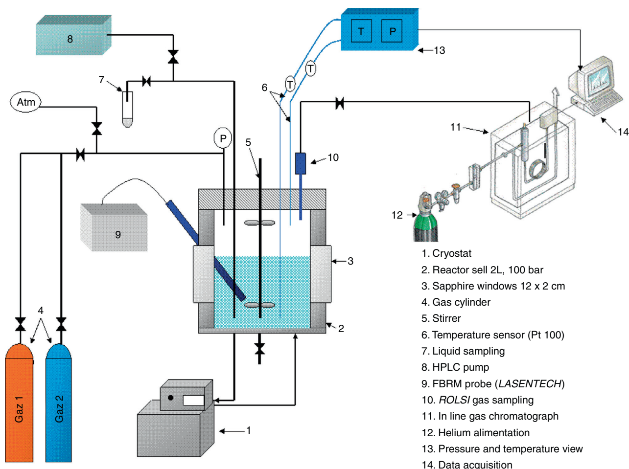
Figure 6 Experimental set-up.
